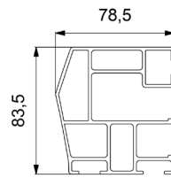
Sideskinne
